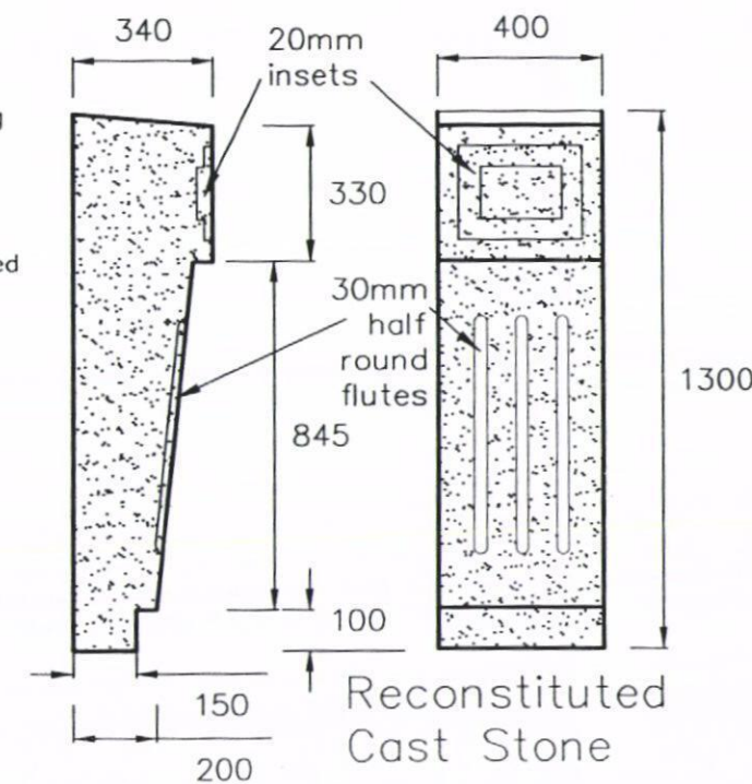
1:20 Bracket
