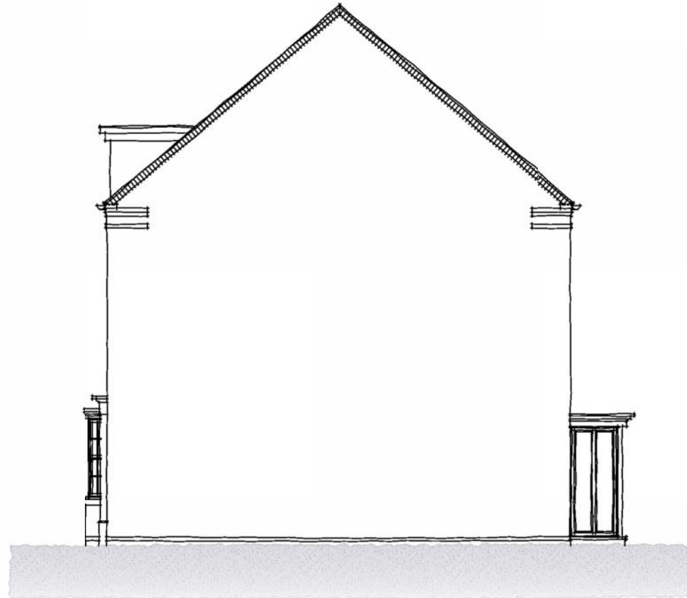
SIDE ELEVATION
