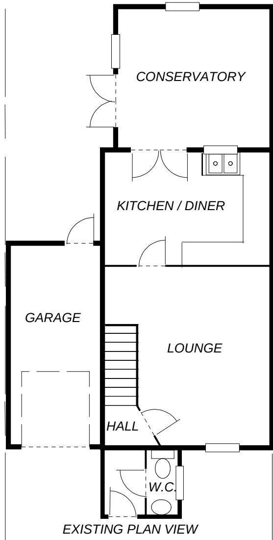
EXISTING PLAN VIEW
