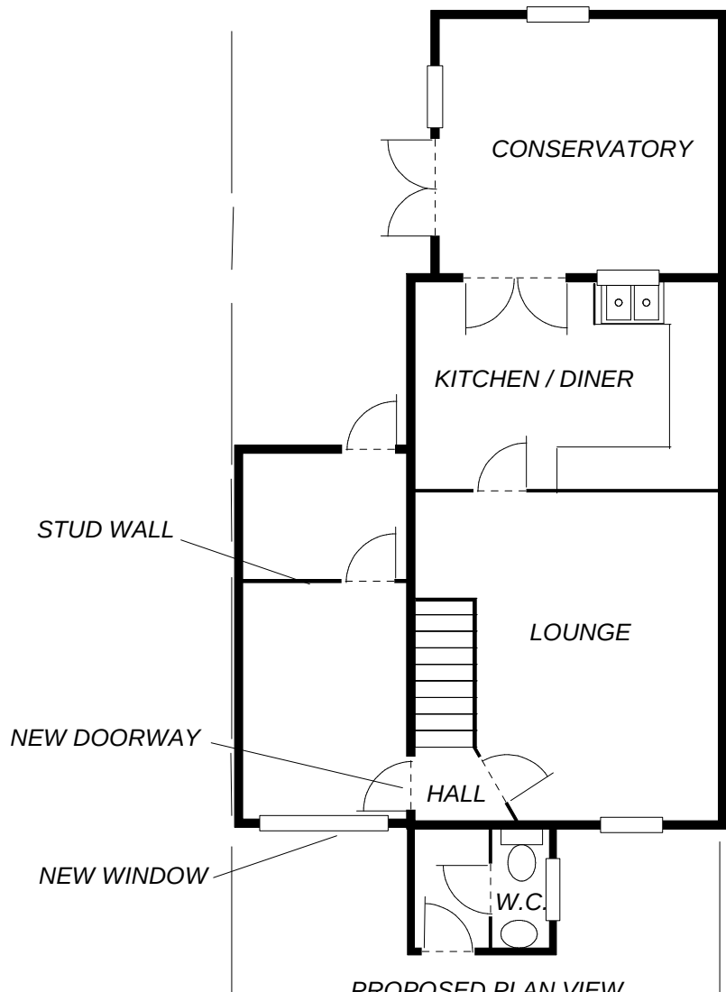
PROPOSED PLAN VIEW
