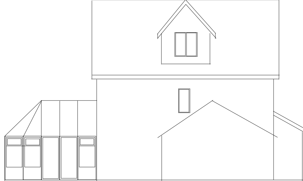
PROPOSED SIDE ELEVATION (East no change)
