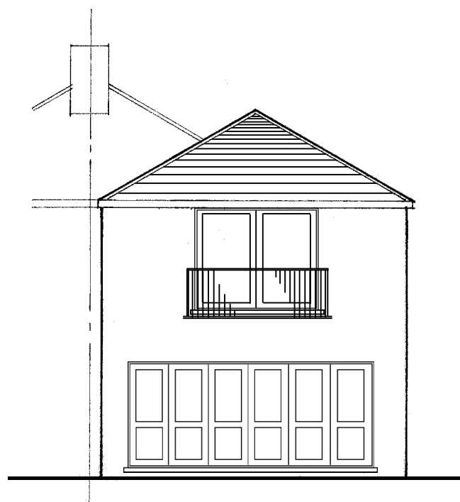
Proposed North/Rear Elevation
