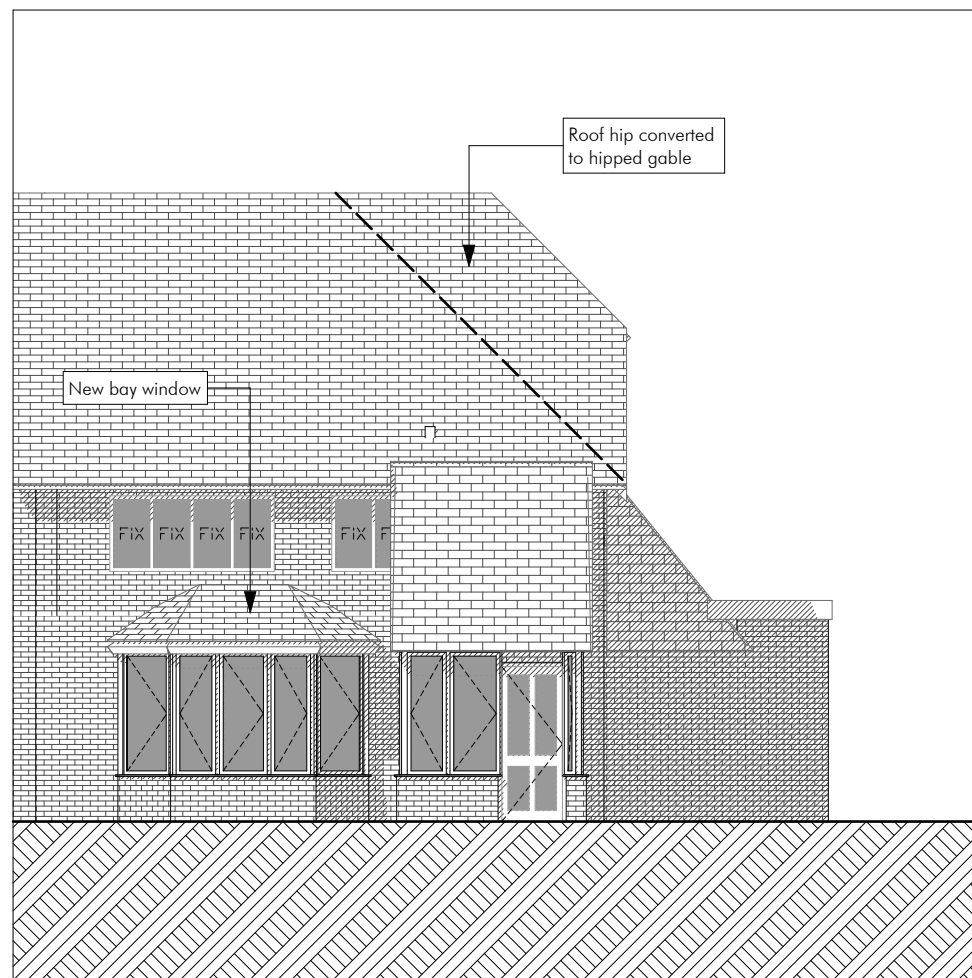
S South Elevation Proposed 1:100
