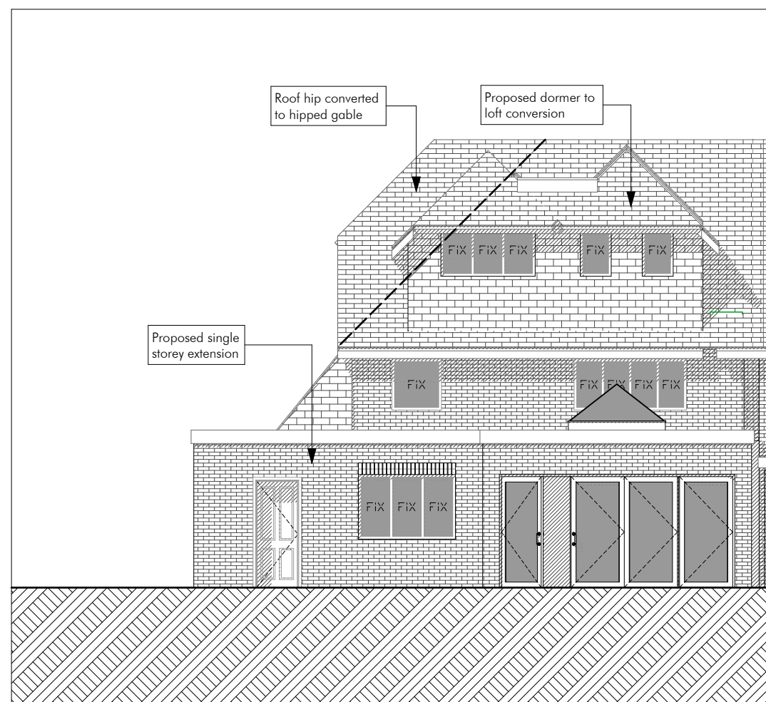
N North Elevation Proposed 1:100
