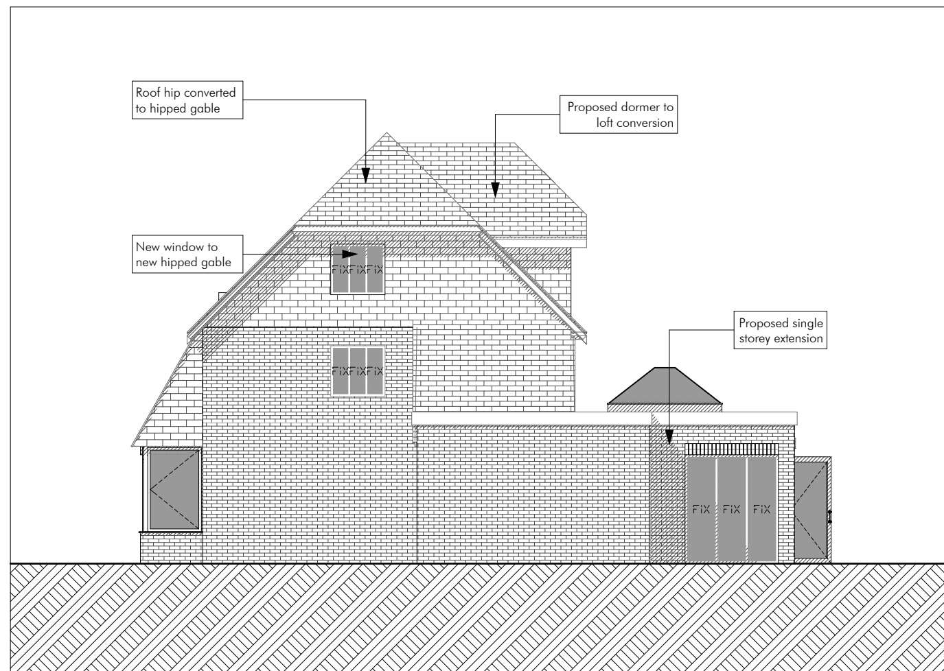
E East Elevation Proposed 1:100
