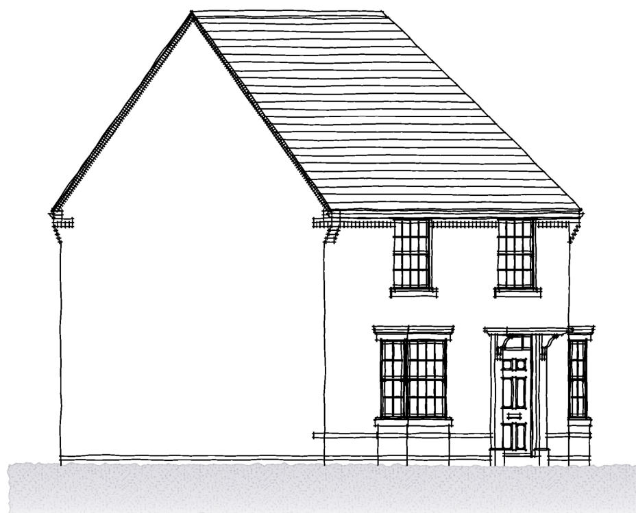
SIDE ELEVATION
