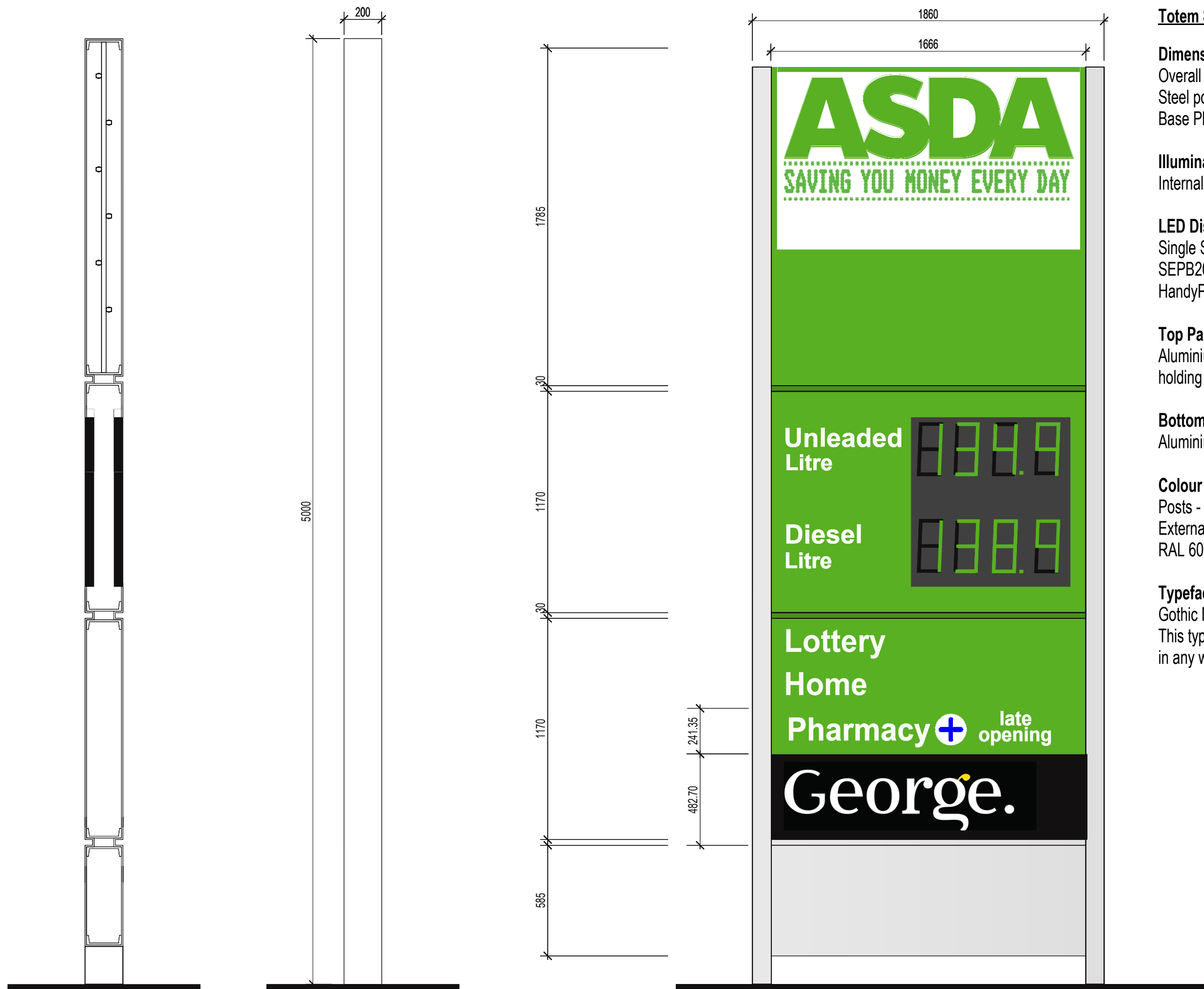
Totem Sign 1: PFS/Store Combined Sign - LED - Scale 1:20 @ A3
