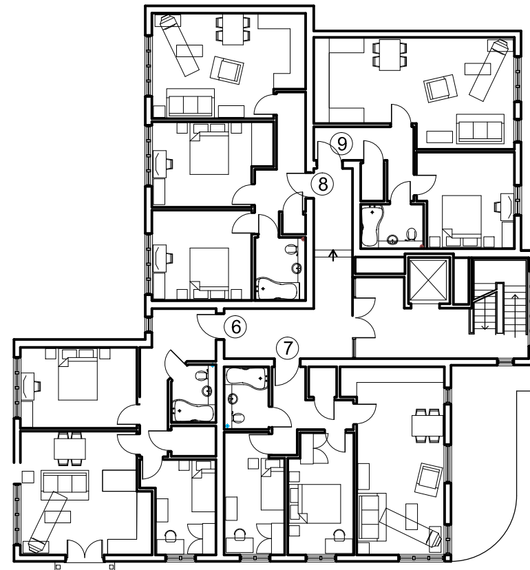
second floor plan (A1 1:100 A3 1:200)
