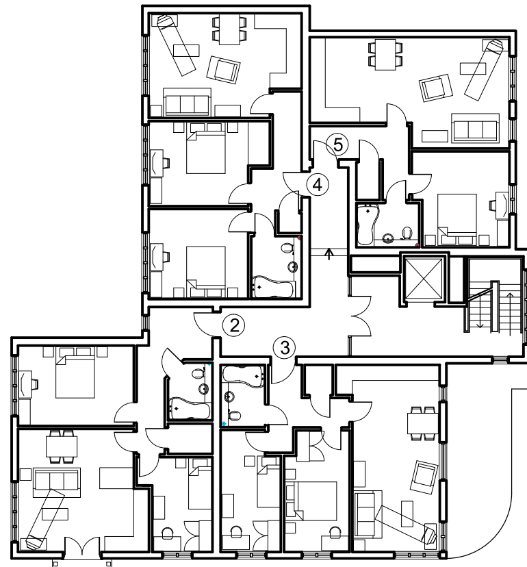
first floor plan (A1 1:100 A3 1:200)
