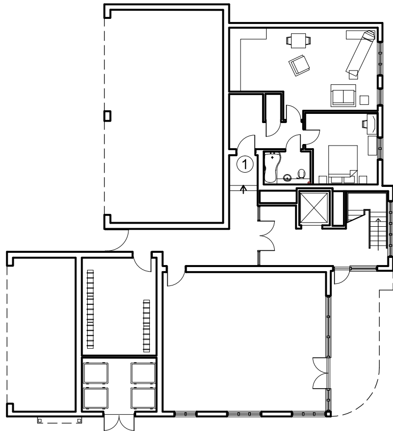
ground floor plan (A1 1:100 A3 1:200)
