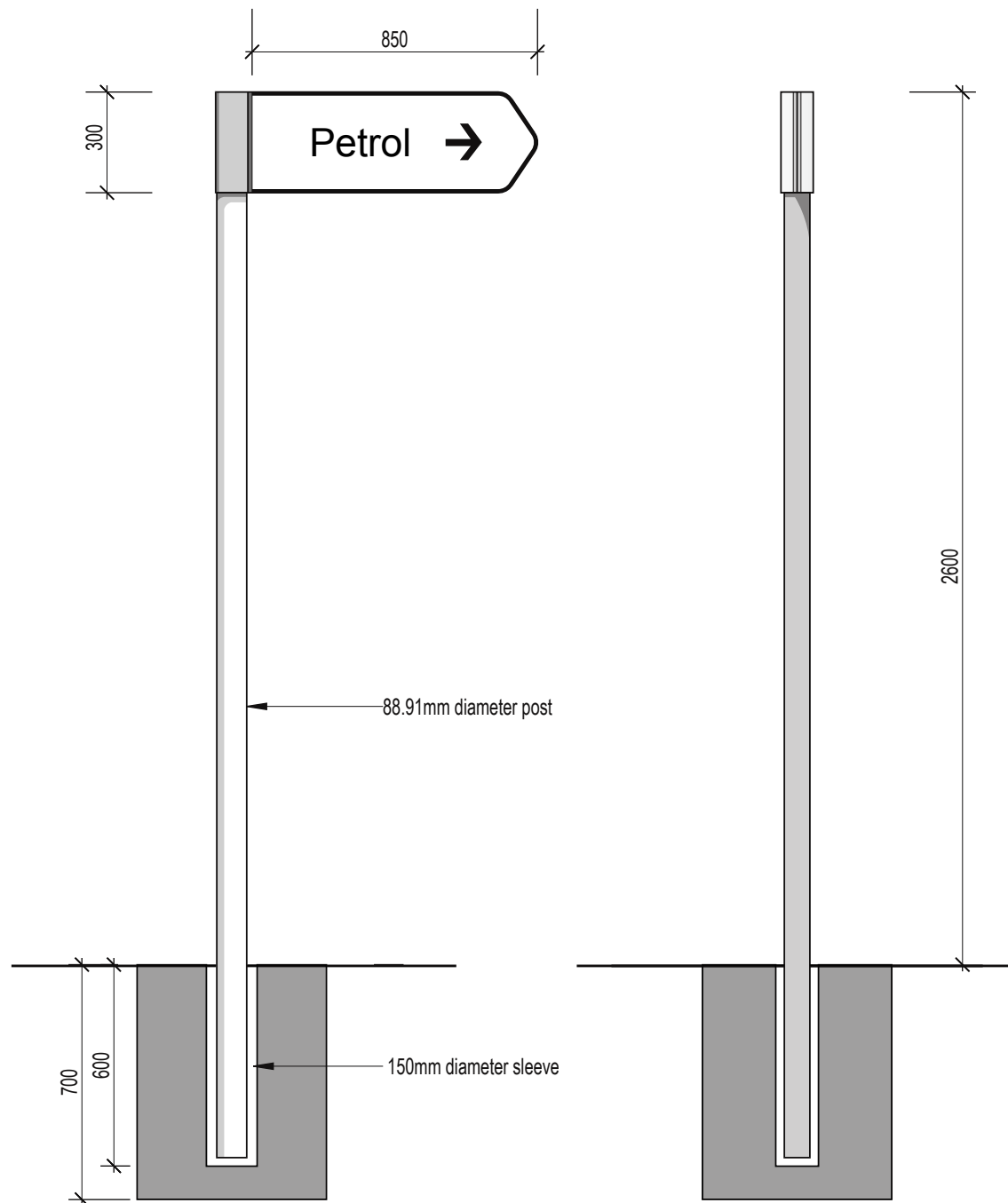
Post Sign 01: Directional "Petrol" - Scale 1:20 @ A4
