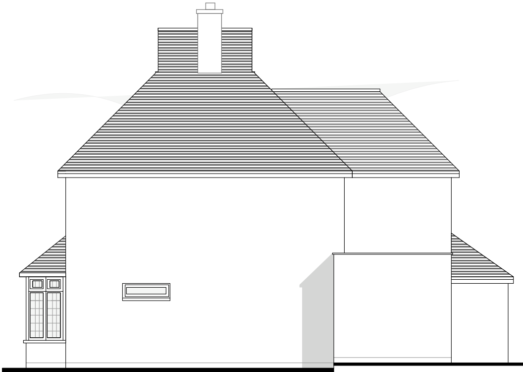
Proposed SOUTH EAST (Side) Elevation at 1:100 scale
