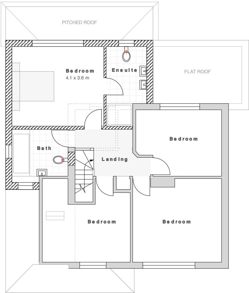
Proposed First Floor Plan at 1:100 scale
