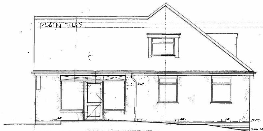
EXISTING SOUTH ELEVATION SCALE 1:100 @ A3
