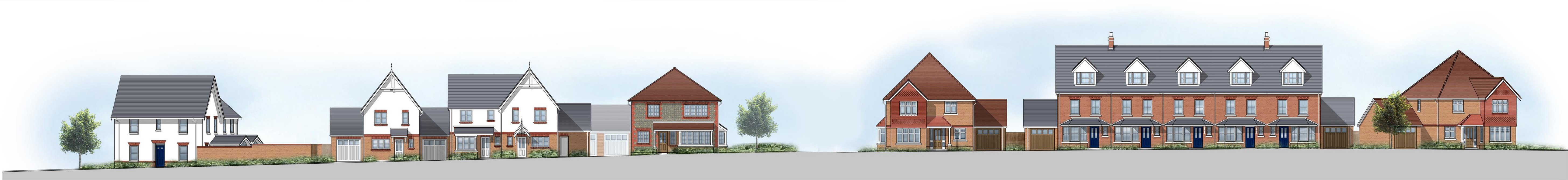
SECTION Y-Y
