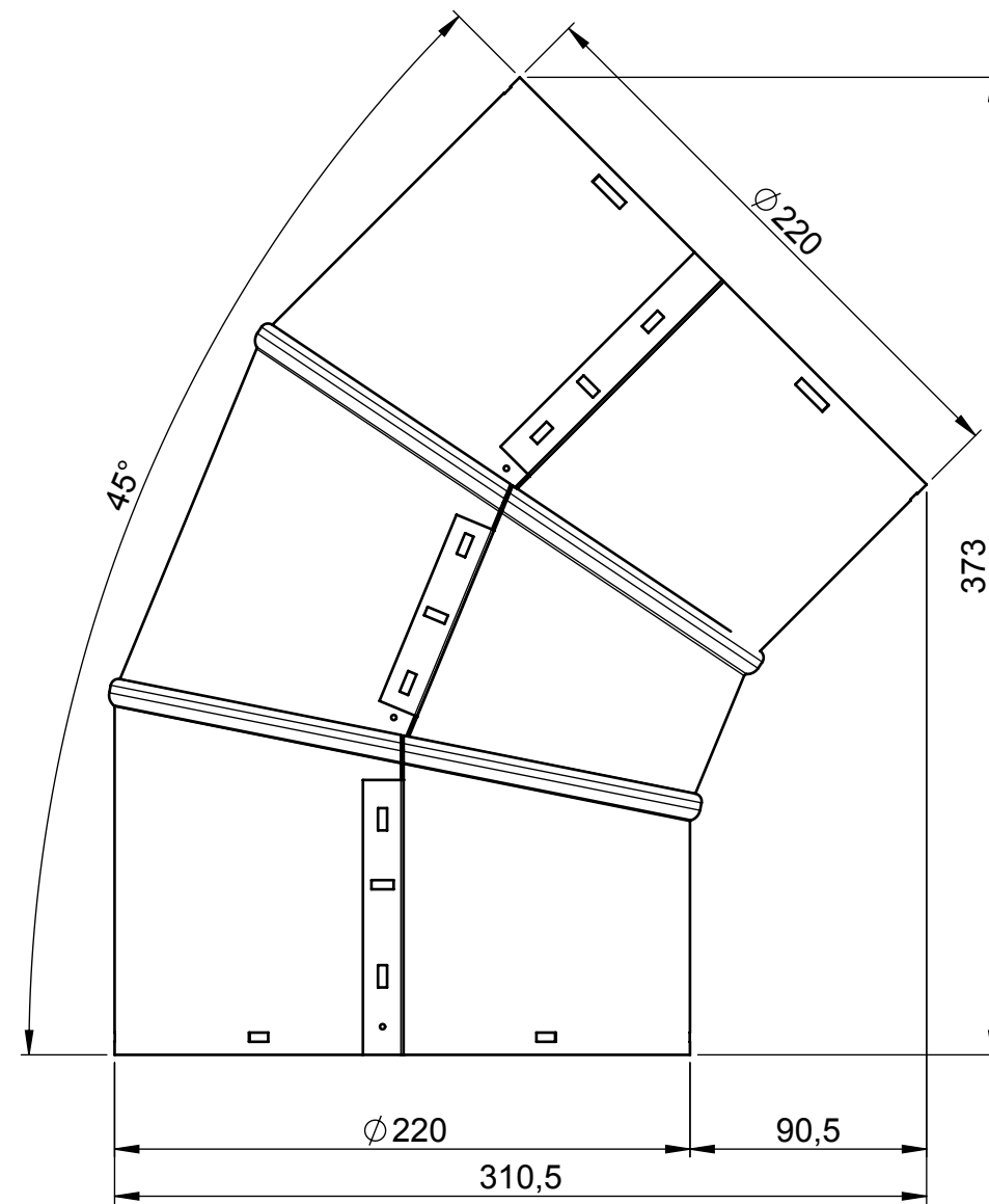
ADJUSTABLE ELBOW 45°
