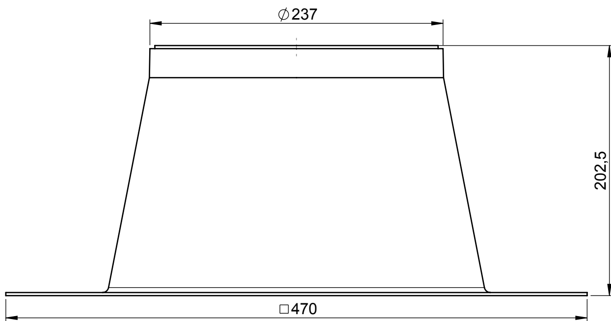
COLLAR
