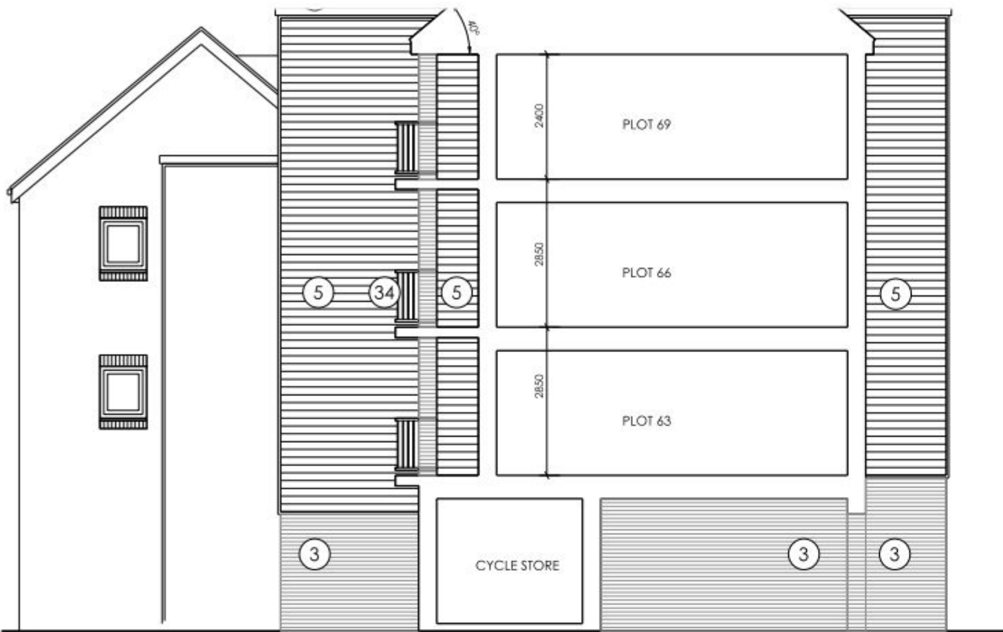
SECTION 2-2 ( NORTH )
