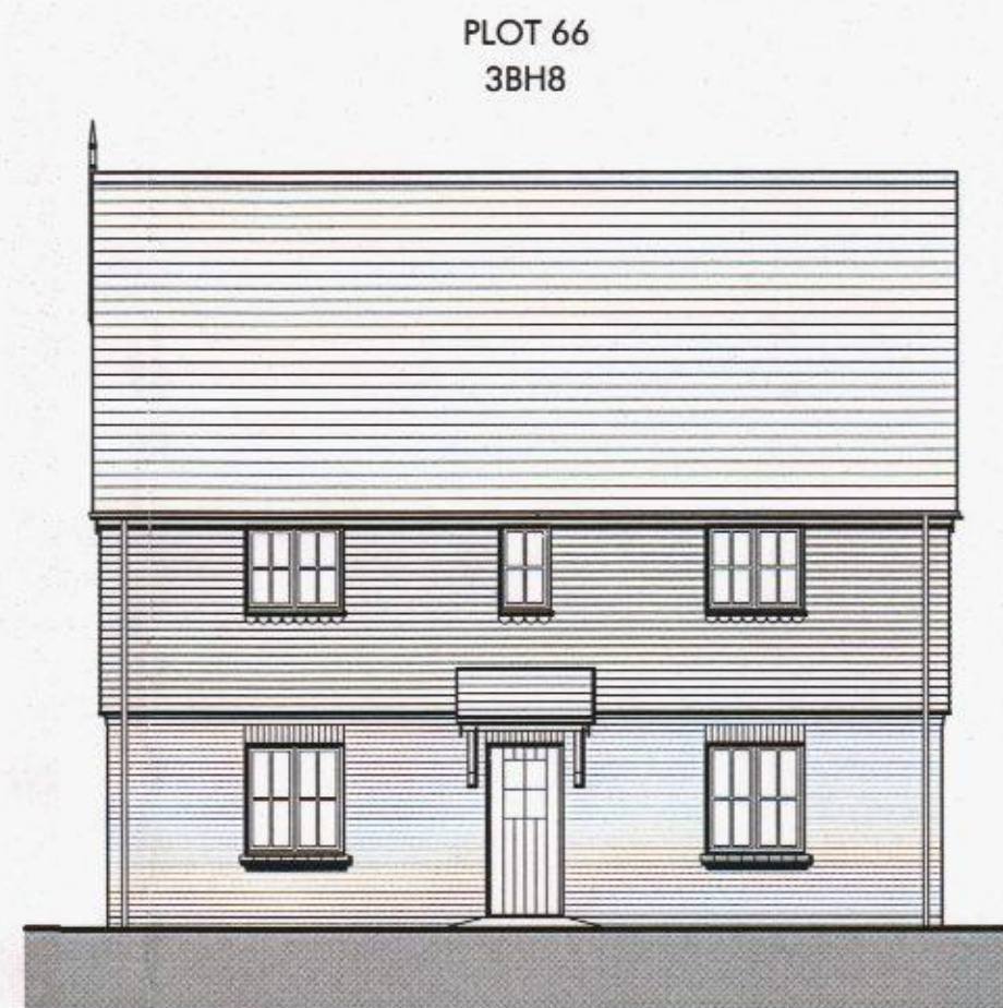
FRONT ELEVATION - A
