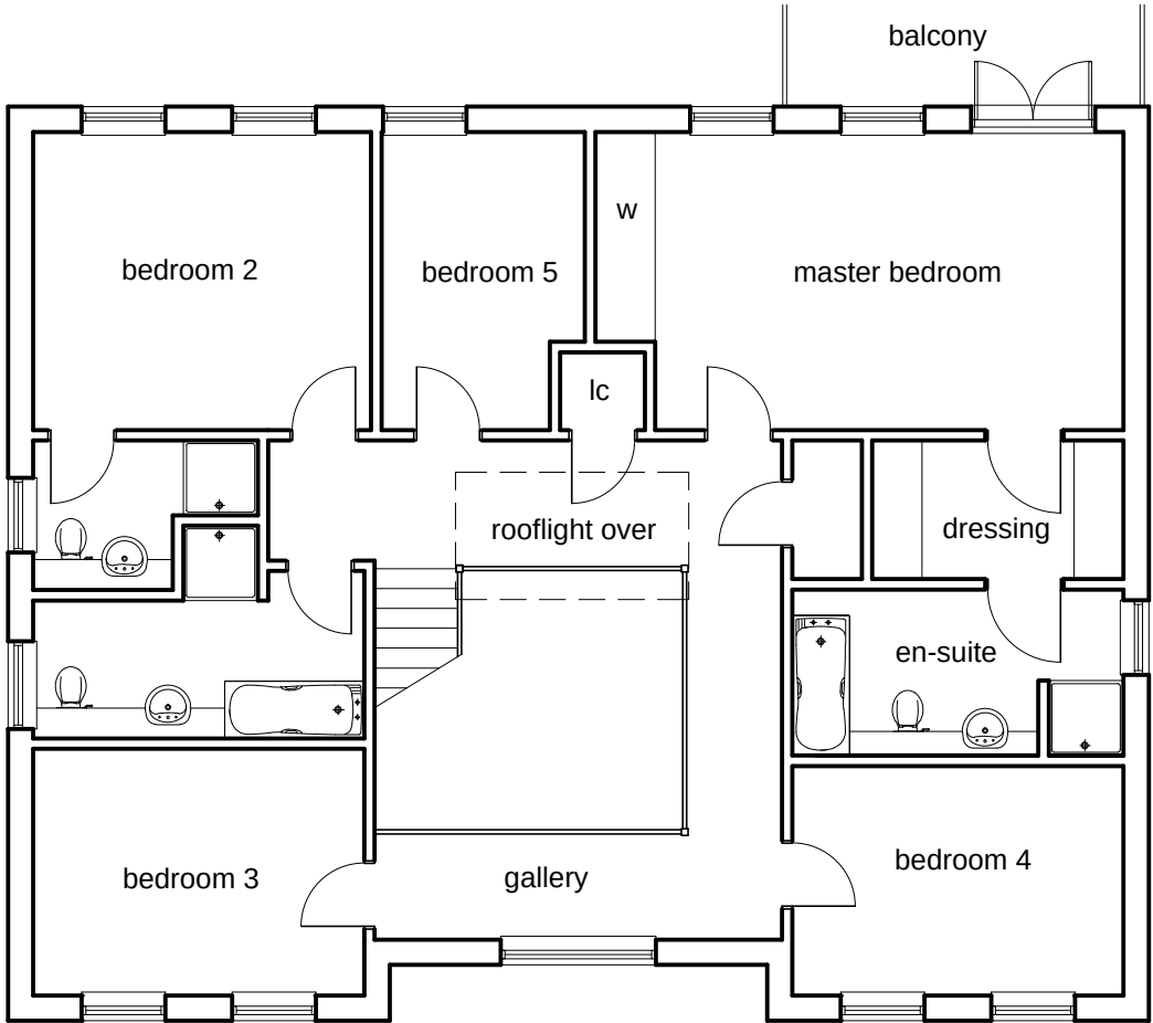
proposed first floor for Units One & Two scale A1 1:50, A3 1:100
