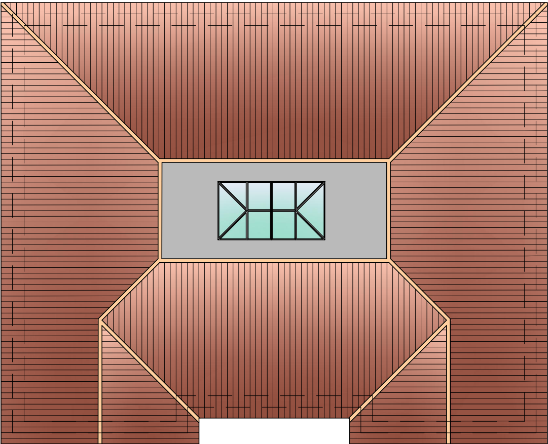
proposed roof plan for Units One & Two scale A1 1:50, A3 1:100
