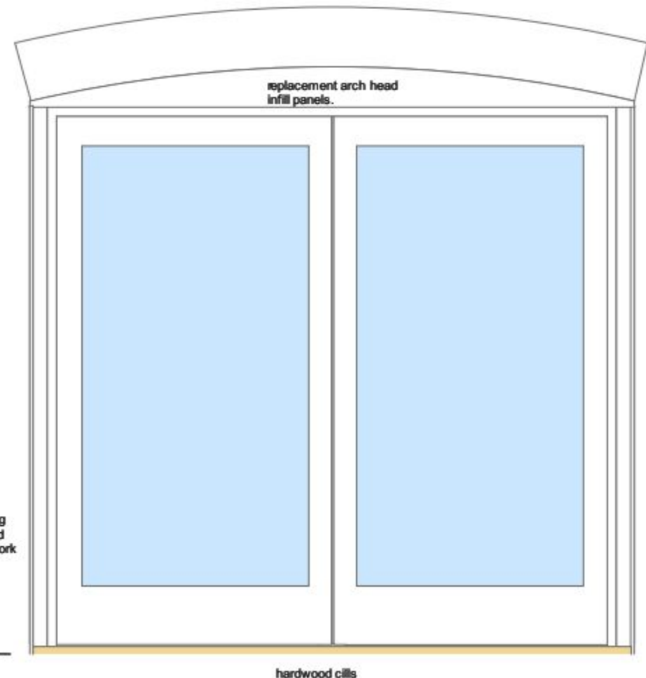
D3 REPLACEMENT DOOR TO SOUTH ELEVATION
