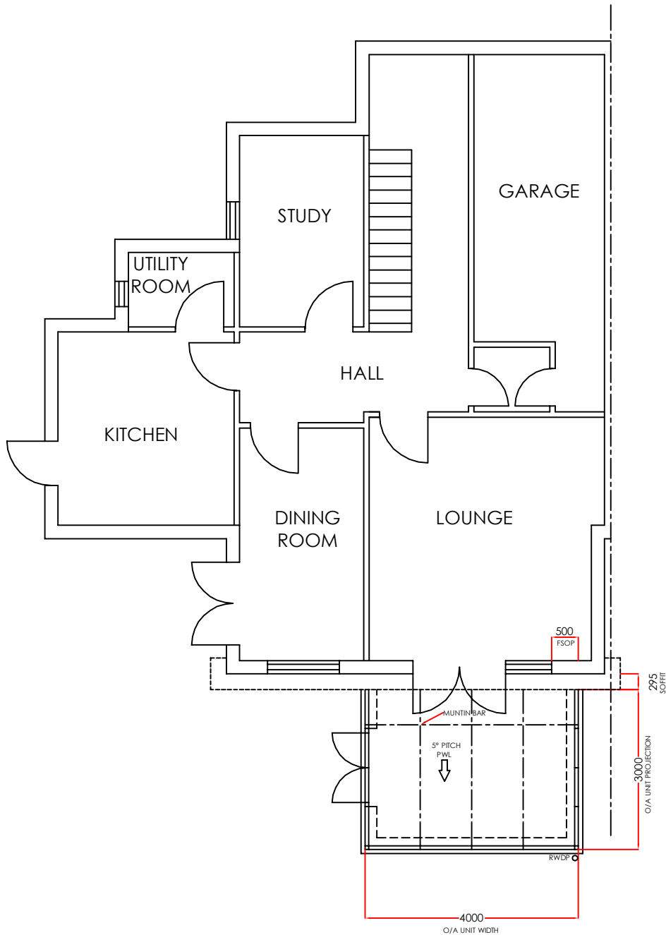
PLAN
