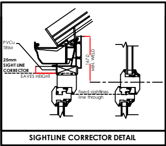
SIGHTLINE CORRECTOR DETAIL
