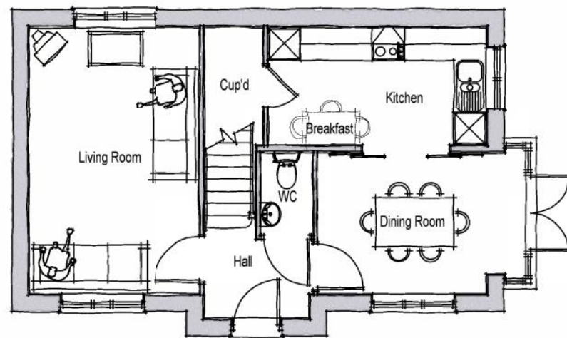
GROUND F
