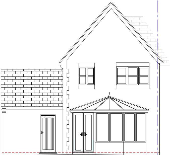
REAR ELEVATION
