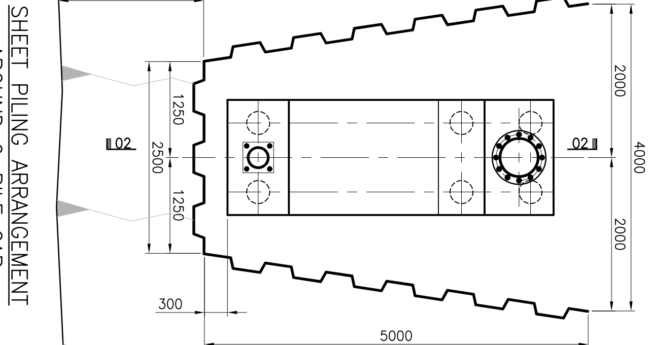
SHEET PILING ARRANGEMENT AROUND 4-PILE CAP SCALE 1:50
