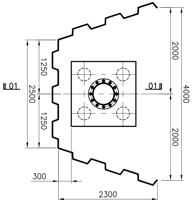
SHEET PILING ARRANGEMENT AROUND 4-PILE CAP SCALE 1:50
