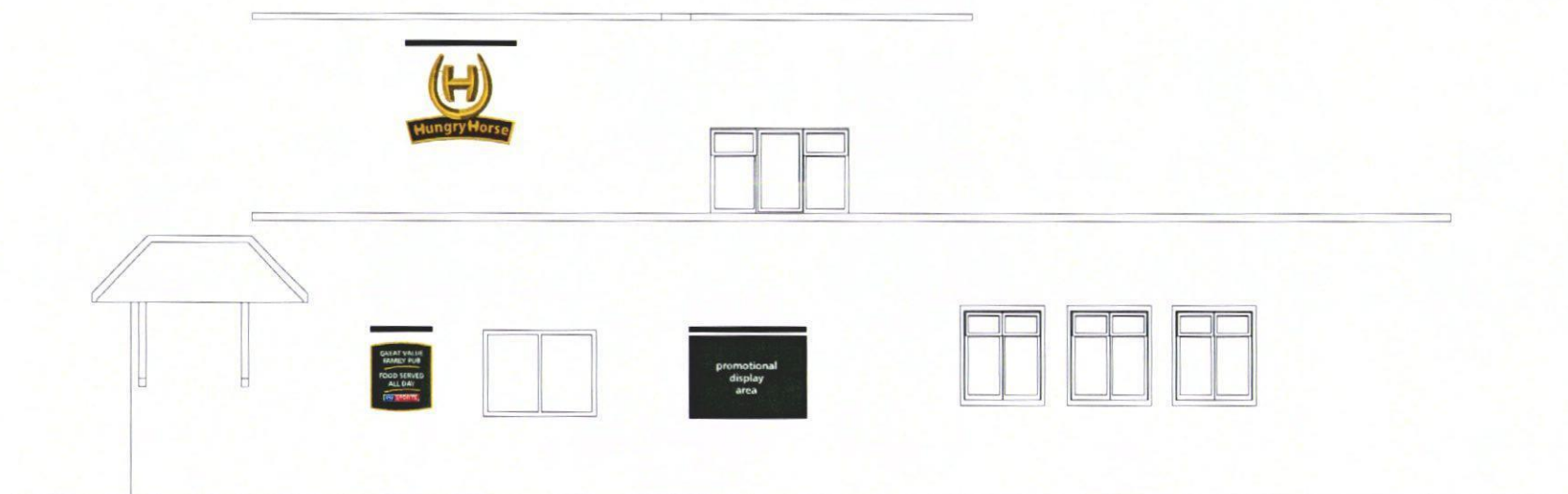
Car Park Elevation - Scale 1:100
