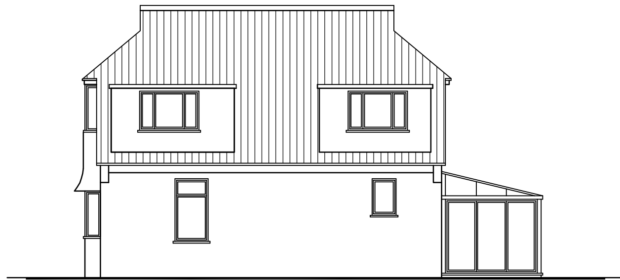
SOUTH
