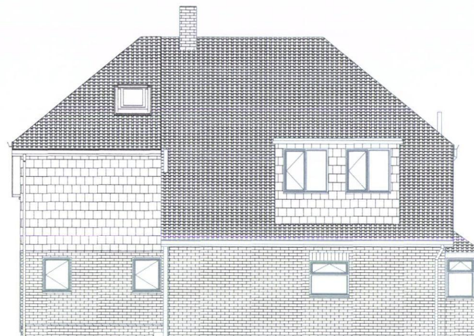
2 ELEVATION SOUTH EAST 1 : 100
