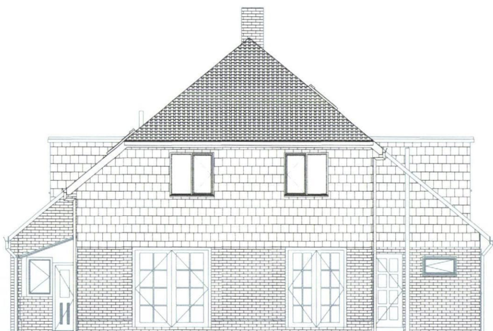
3 ELEVATION SOUTH WEST 1 : 100
