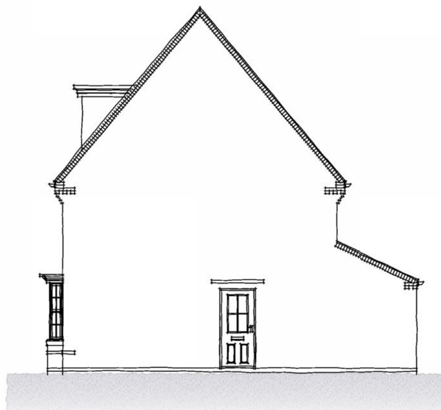
SIDE ELEVATION
