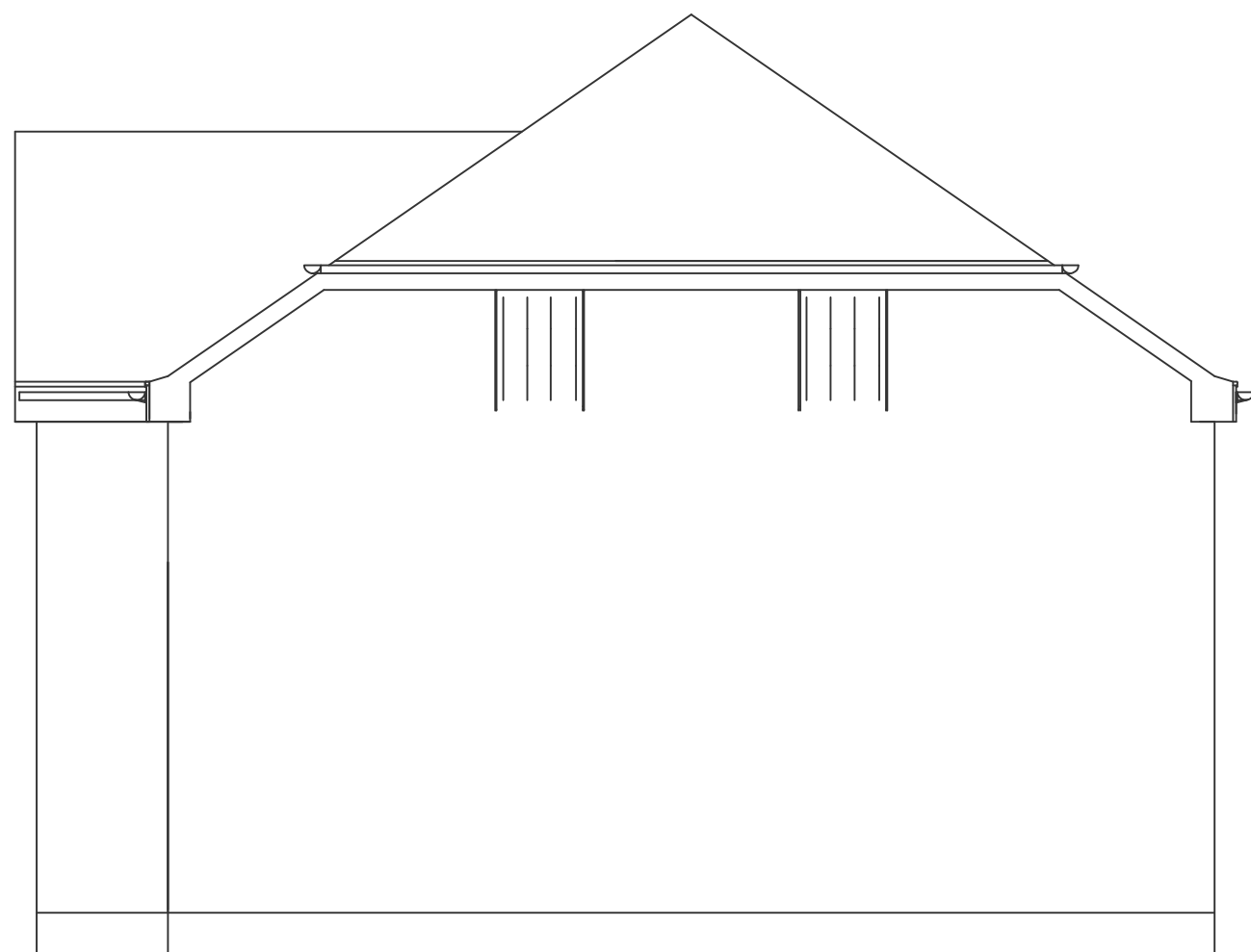
MIDDLE BARN EXISTING EAST ELEVATION
