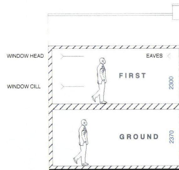
Section at 1:100 scale
