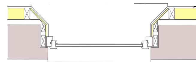
PLAN OUTSIDE
