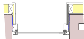
PLAN OUTSIDE
