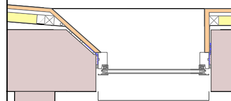
PLAN OUTSIDE
