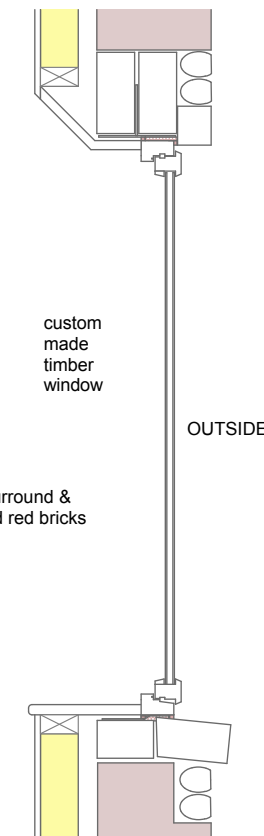
SECTION
