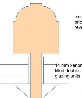
DETAIL
