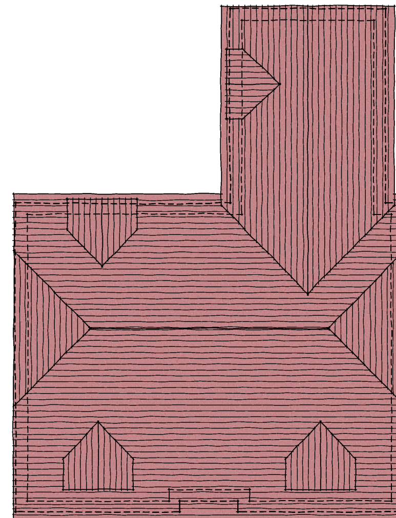
ROOF PLAN
