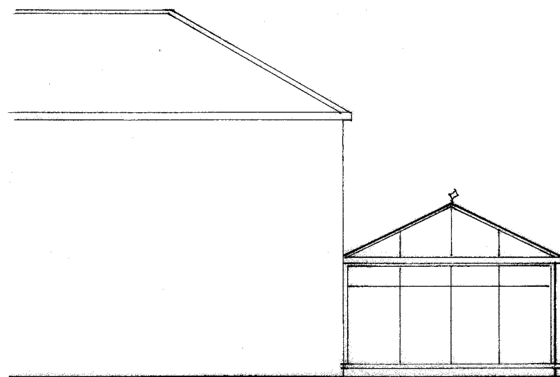
Proposed South/Side Elevation
