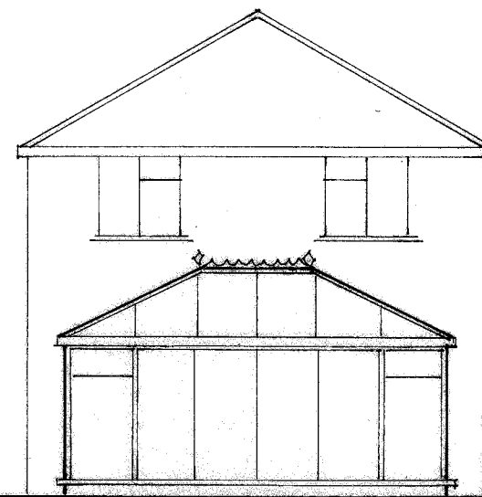
Proposed East/Rear Elevation
