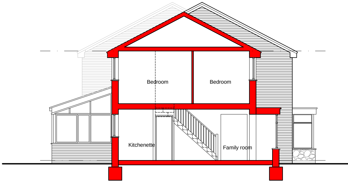
Proposed Side Extension
