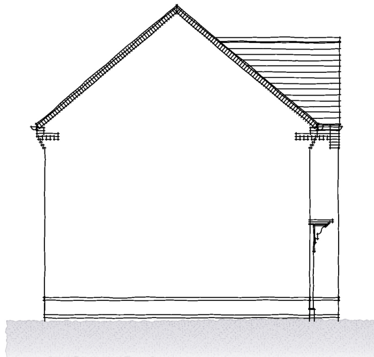
SIDE ELEVATION
