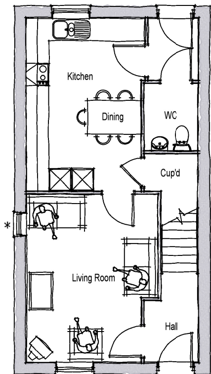
GROUND FLOOR PLAN * WINDOW TO PLOTS 65 & 86 ONLY
