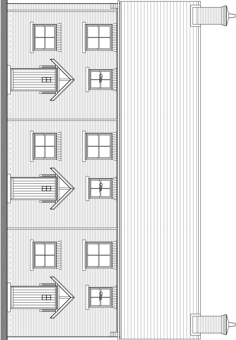
Front Elevation
