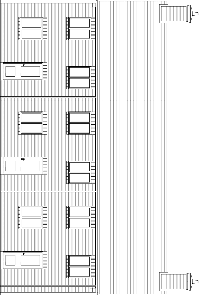
Rear Elevation
