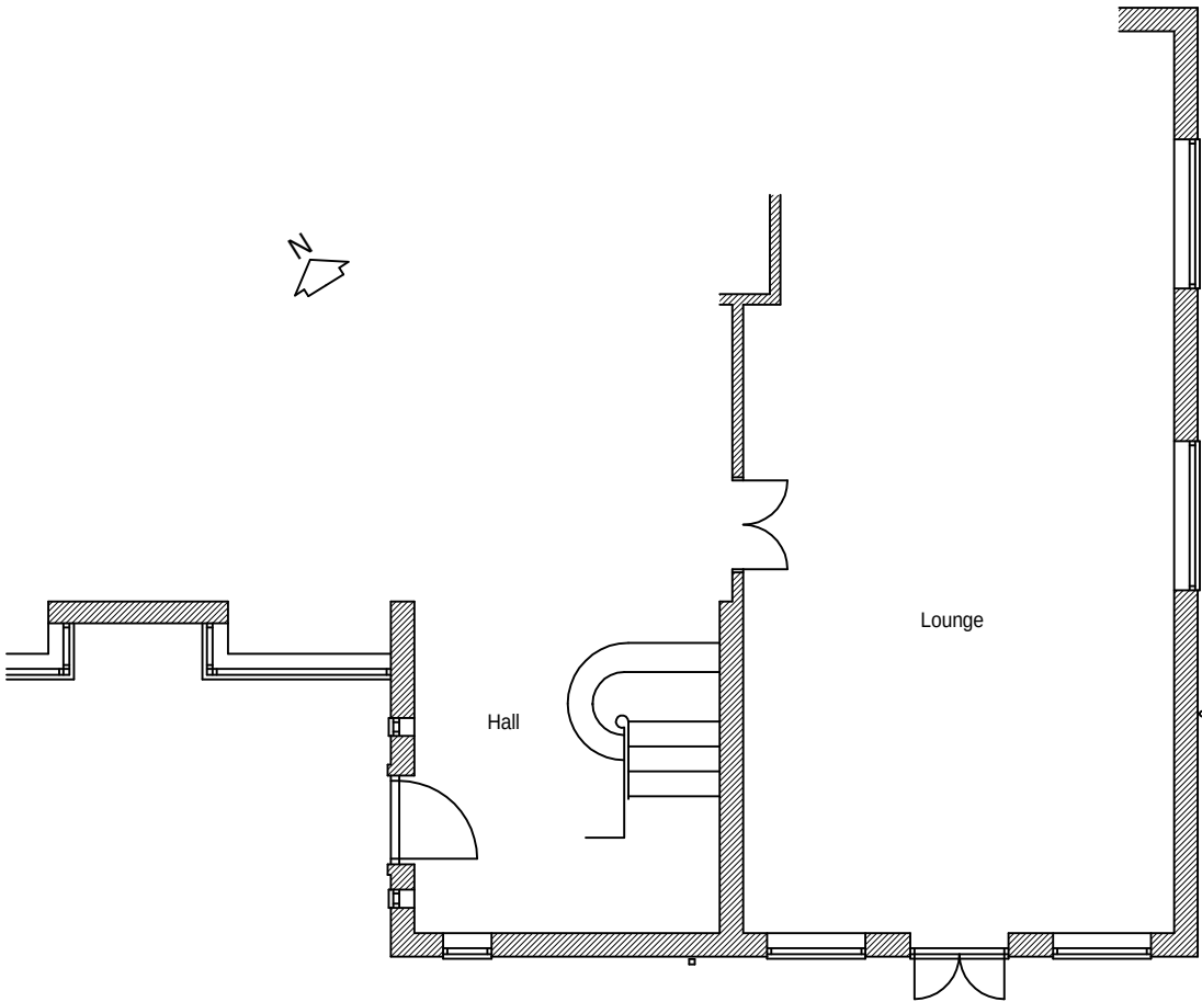
Part Existing Ground Floor Plan (south-east corner)
