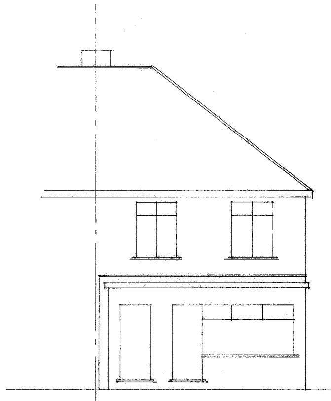
Existing SE/Rear Elevation
