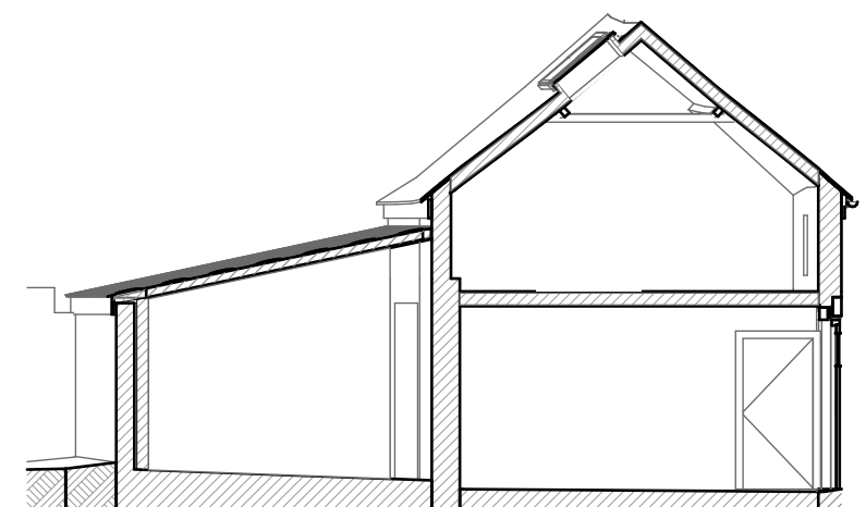
CROSS SECTION LOOKING TO EAST: AS EXISTING
