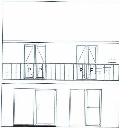
Existing NW Elevation
