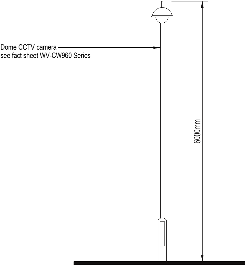
CCTV Camera
