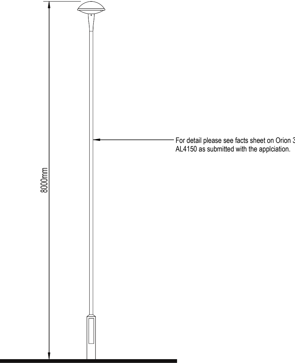
Lighting Column
