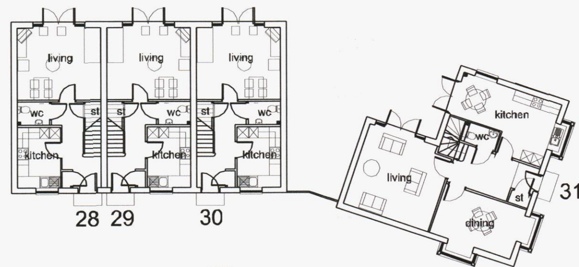
ground floor plans plots 28-31
