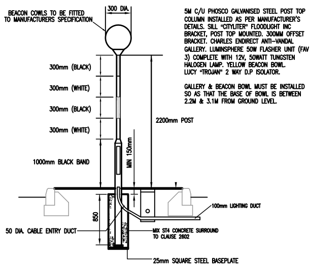
2.5m BELISHA BEACON DETAIL
