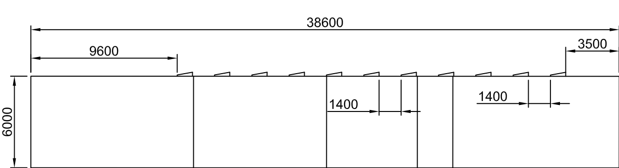
1:250 ELEVATION A
