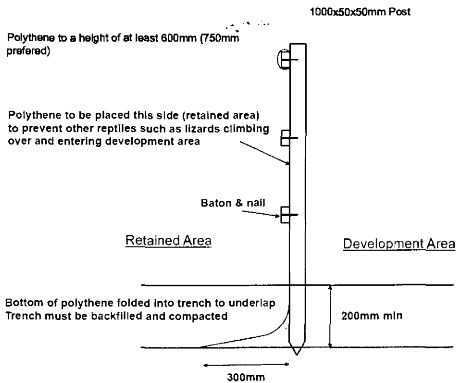
Figure 6. Specifications of reptile exclusion fencing.
