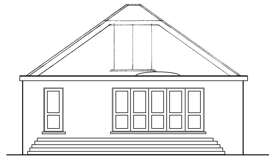
Proposed NE/Rear Elevation
