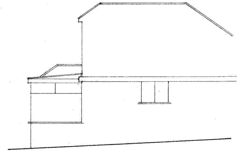
Existing NW/Side Elevation
