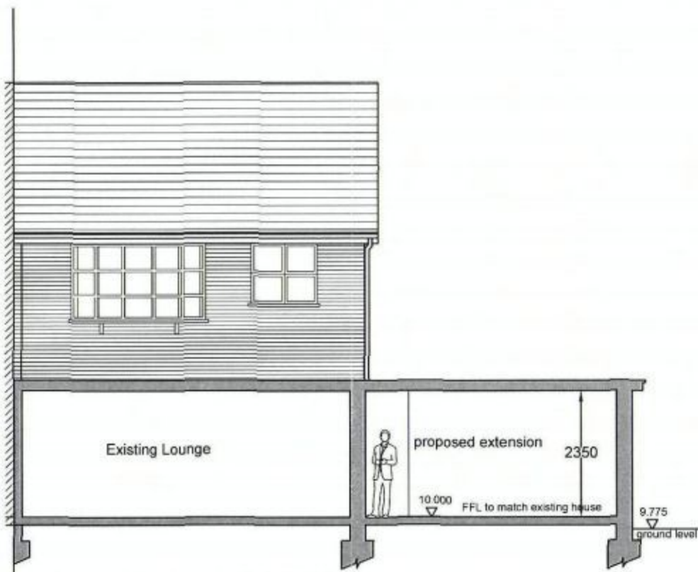
Proposed Section - Scale 1:100 @ A3
