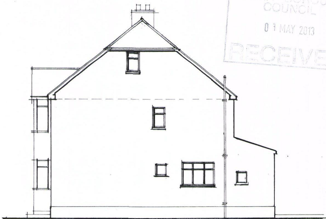
EAST ELEVATION
