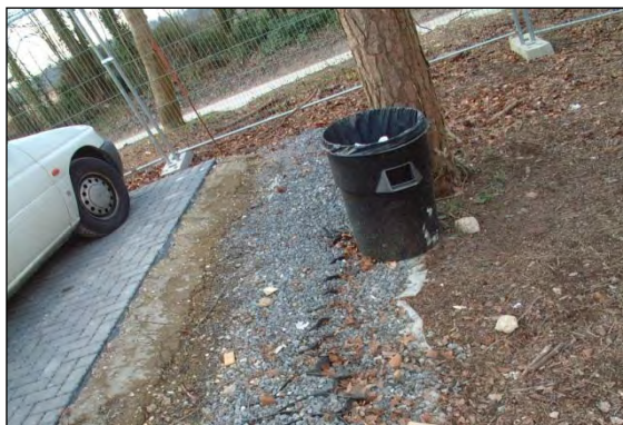
Photo 26: A conventional concrete haunching can be used to retain new surfacing as long as it is not dug into a trench - here is it placed on top of the CellWeb layer.
