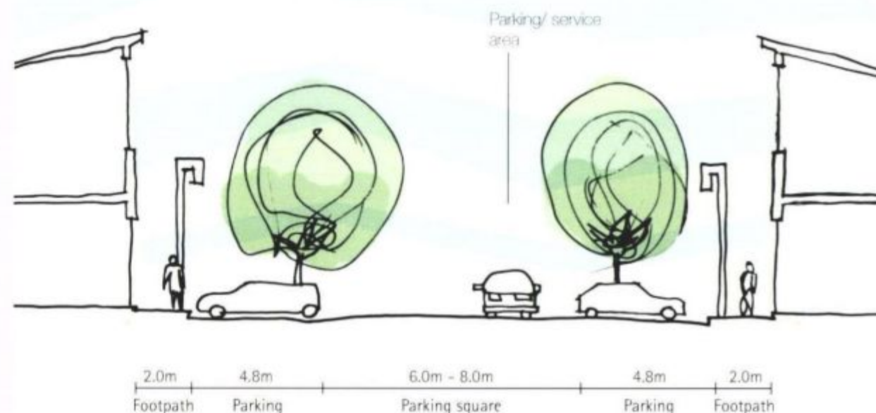
Employment courtyard - allowing for servicing and parking. Designed as a space and formally lit
