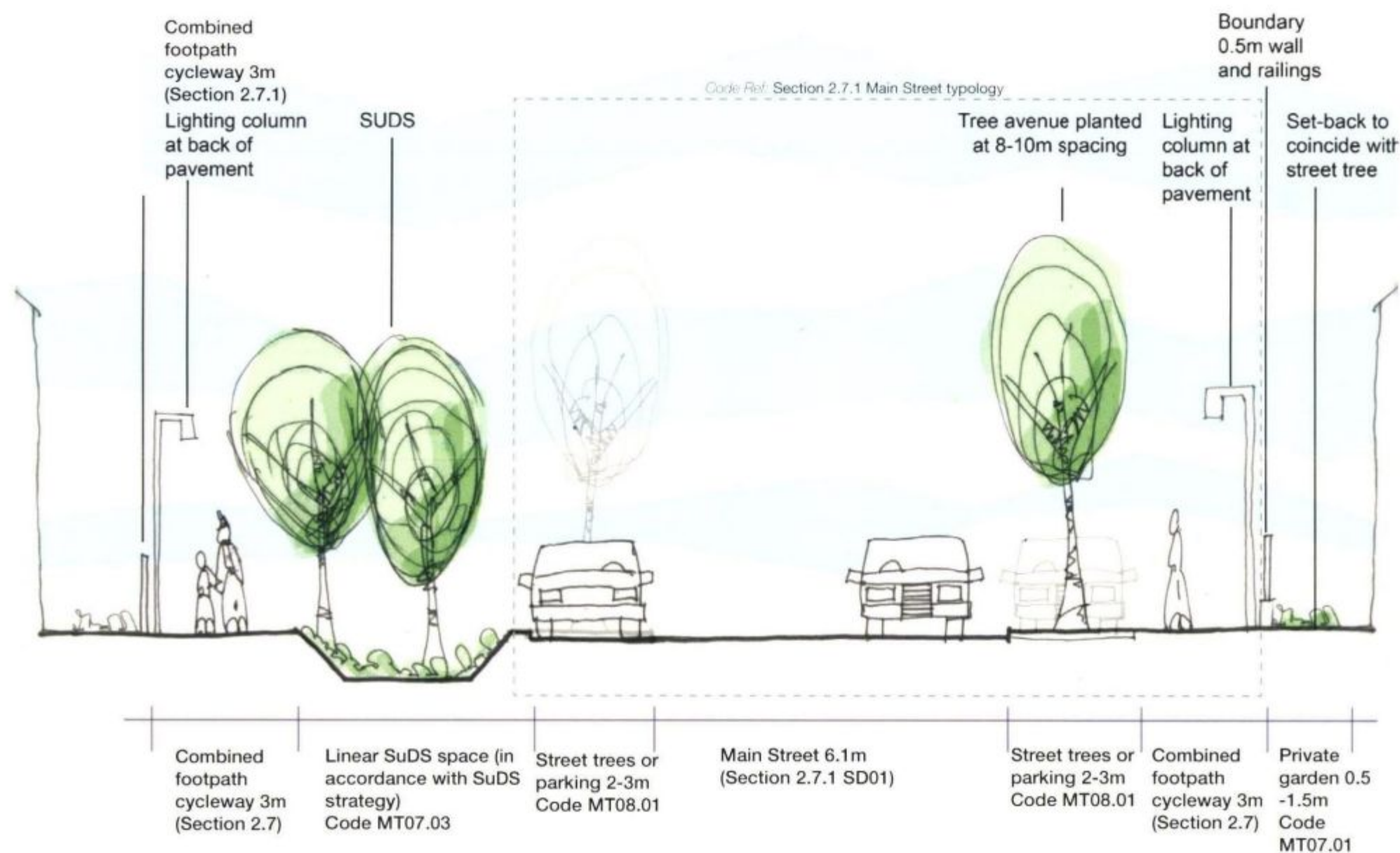
MT4 Section
