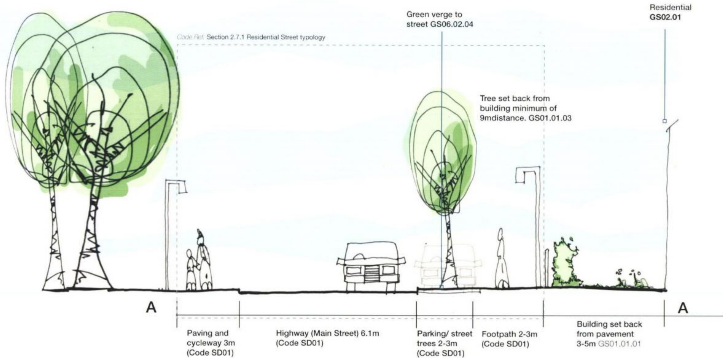
GS3 Section
