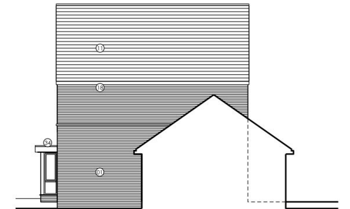
SIDE ELEVATION (PLOT 16)
