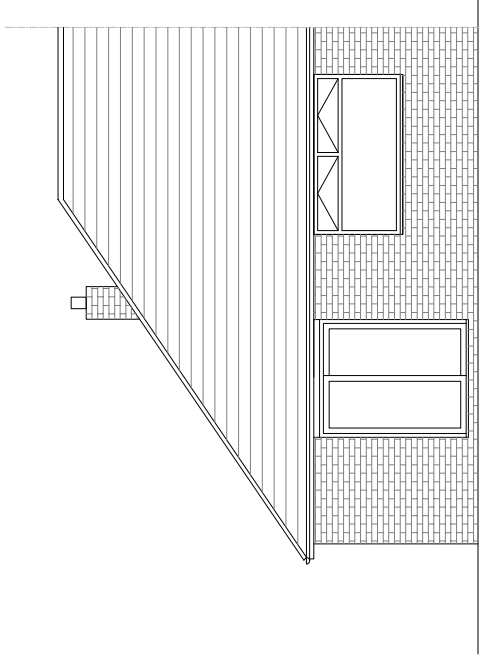
Existing Rear Elevation (Without Existing Conservatory)
