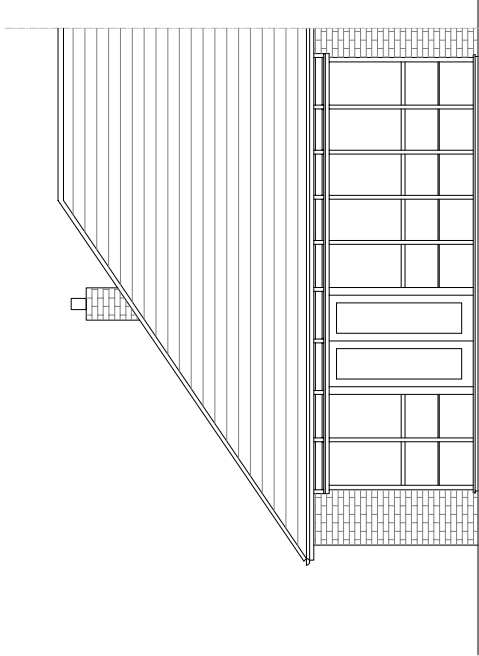
Existing Rear Elevation (Showing Conservatory)
